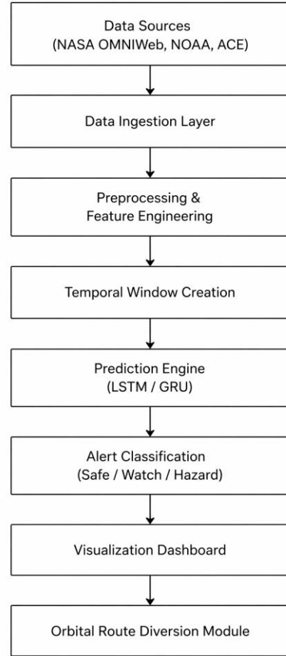
FIGURE I SYSTEM ARCHITECTURE OF COSMOPREDICT
